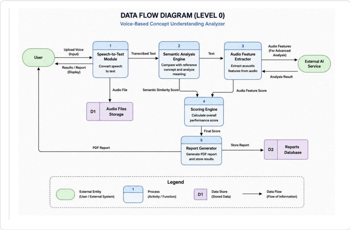
Figure 1: Data Flow Diagram of Voice-Based Concept Understanding Analyzer
